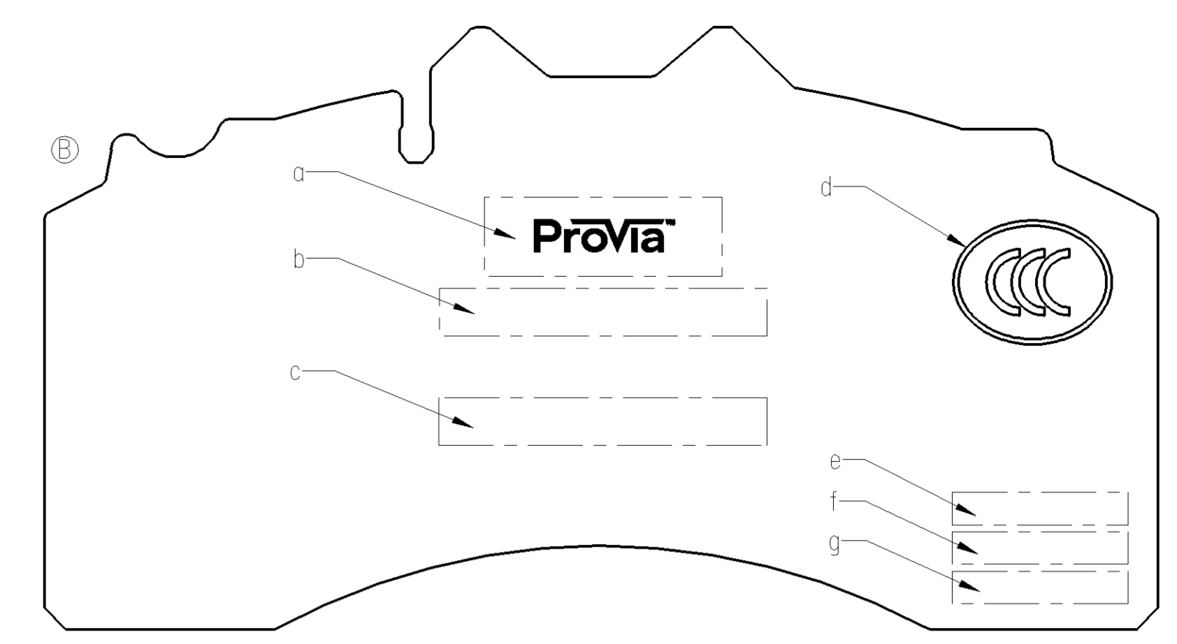
MARKING ON BACKING PLATE - DRAFT ONLY FOR EXPLANATION OF THE TEXT AREAS. BACKING PLATE CONTOUR, SIZE AND ALIGNMENT OF AREAS MAY DIFFER FROM THE REAL PART.
