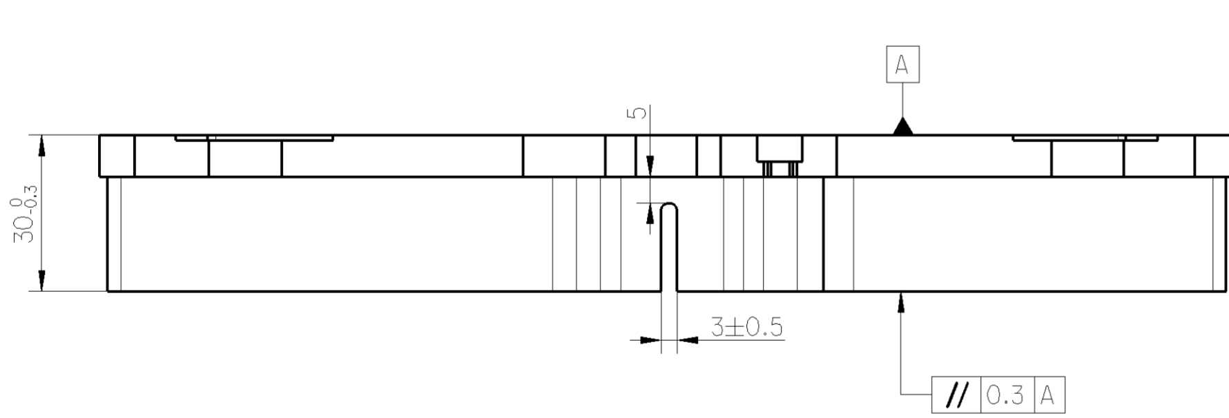
PROJECTION WITHOUT LEAF SPRINGS
