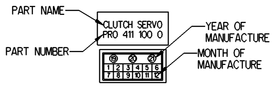
6 STICKER DETAILS
