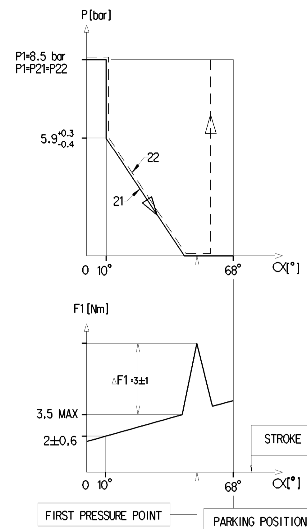
DELIVERED PRESSURE DIAGRAM
